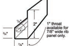
LG 132 COMBO TRACK COVER
