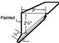
LG 131 NATIONAL DOOR TRACK COVER
