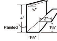
LG 133 TOP MOUNT TRACK COVER
